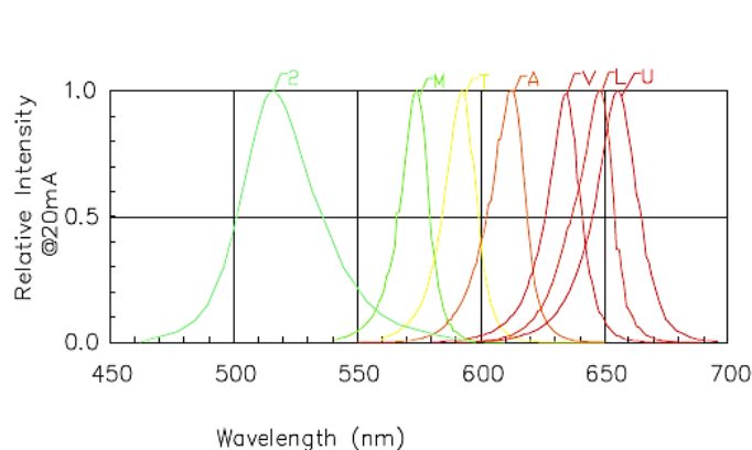
Fig 5. Relative Intensity vs. Wavelength
